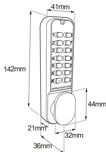
BL2000 - Internal Keypad
