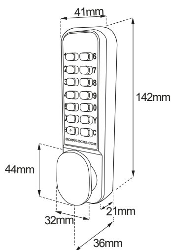
BL2000 ECP - Keypad only
