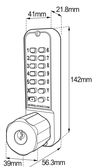
BL2700 ECP - Internal Keypad
