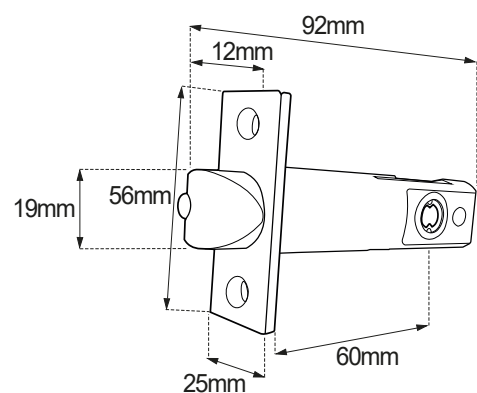
60mm tubular latch - 2000 Series
