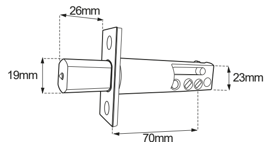
Mortice deadbolt - Extended
