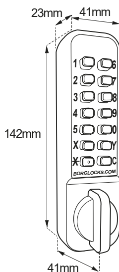
BL2107 ECP - External Keypad
