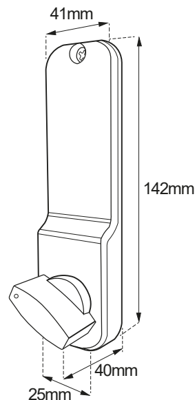
BL2107 ECP - Internal handle
