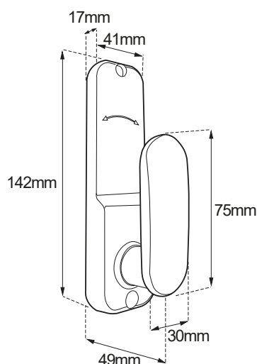
BL2000 ECP - Inside handle
