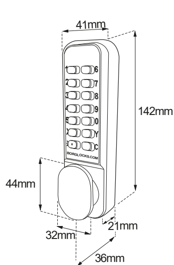
BL2000 ECP - Keypad only
