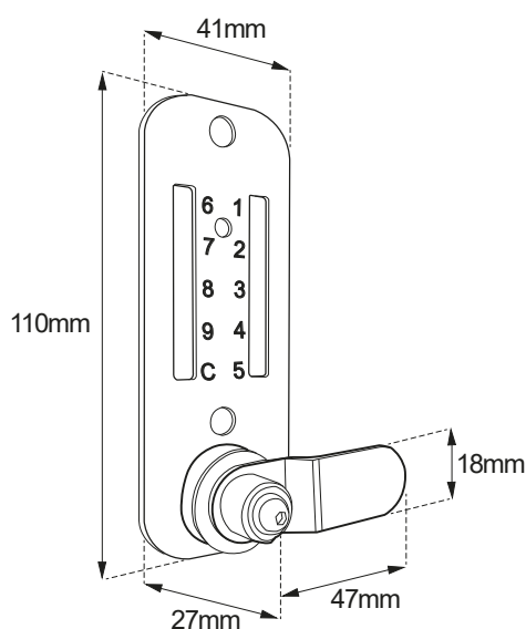
BL1500 ECP - Internal cam
