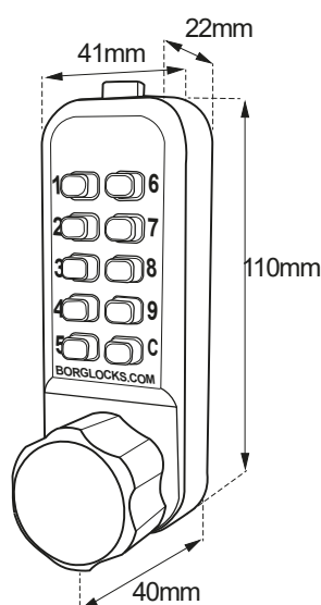
BL1500 ECP - External Keypad
