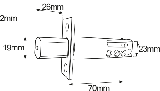
Mortice deadbolt - Extended
