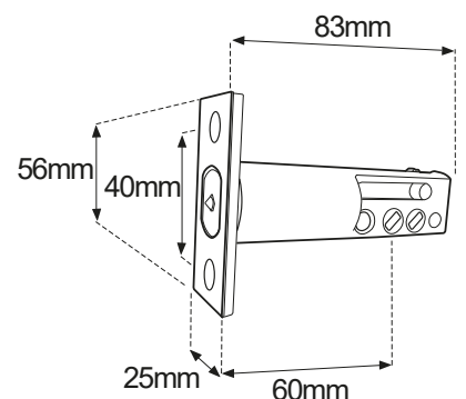
Mortice deadbolt - Retracted
