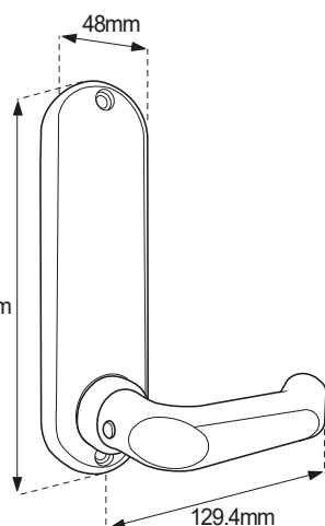
BL5000 ECP Inside handle
