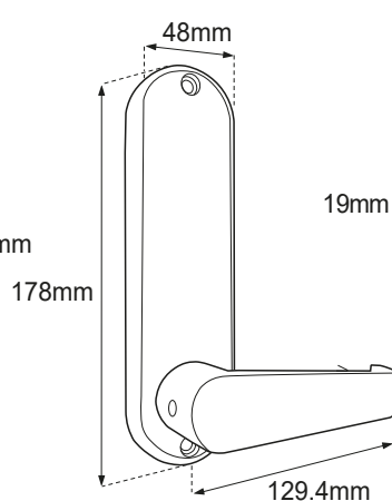
BL5700 ECP - Inside handle
