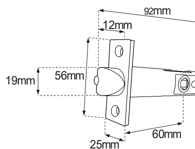
60mm tubular latch - BL5000 Series
