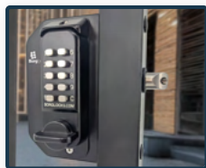
BL3030 ECP - Back to back gate lock for use with 40-60mm box sections
