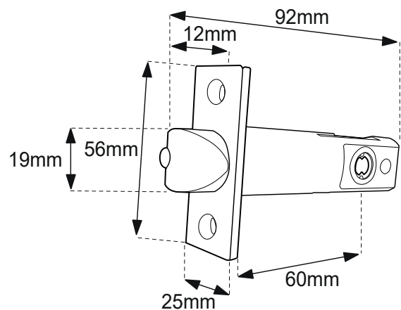
60mm tubular latch - 2000 Series
