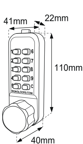
BL1500 ECP - External Keypad
