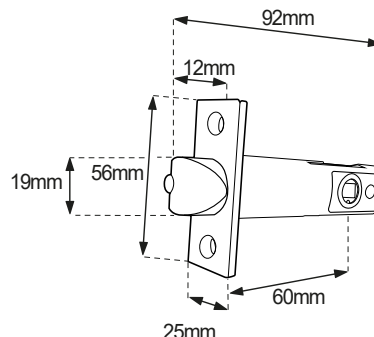
60mm tubular latch
