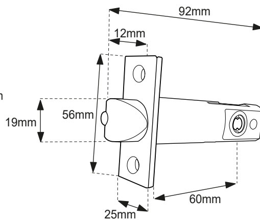
60mm tubular latch
