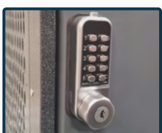
BL1706 ECP - Single sided keypad w/ internal cam lock and key override
