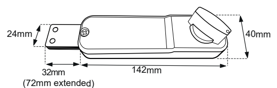
BL2615 ECP Inside deadbolt
