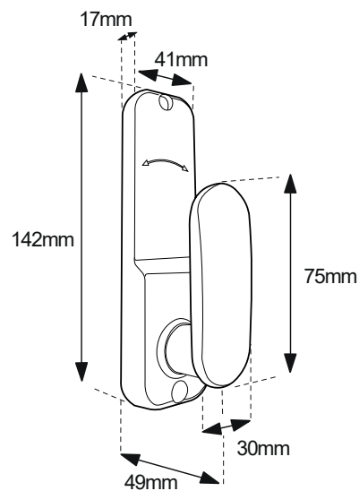
BL2000 ECP - Inside handle
