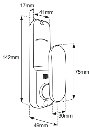
BL2601 ECP Inside handle
