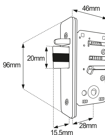
28mm ali latch BL5000 Series
