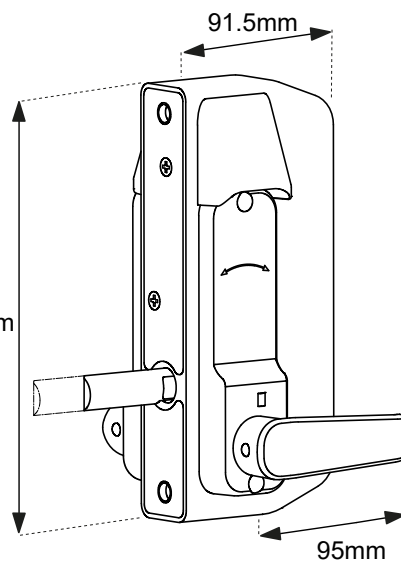
BL3400 ECP Inside handle
