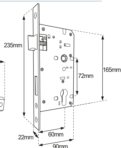
60mm backset euro sash lock
