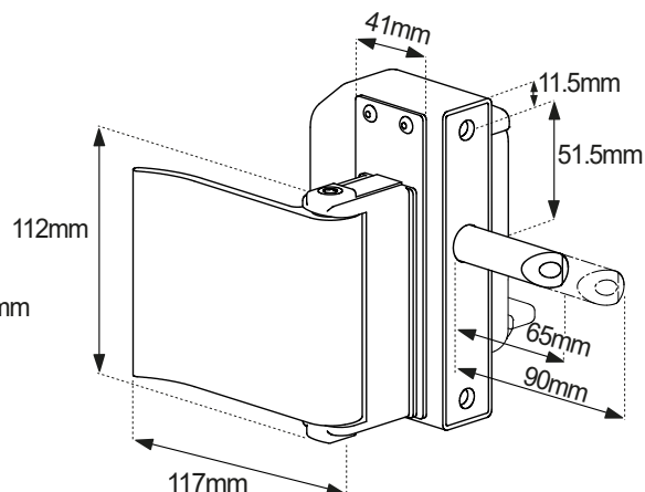
BL3080 ECP Push/pull pad
