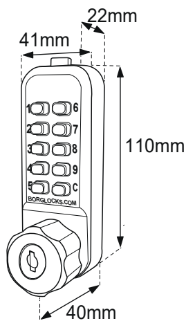
BL1700 ECP - External Keypad
