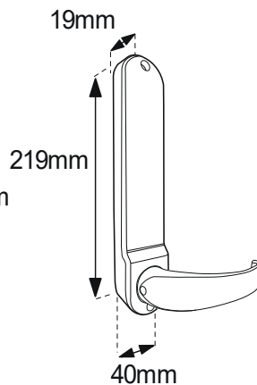
BL6000 ECP - Internal Handle
