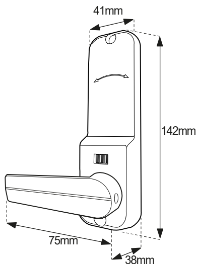
BL2400 ECP - Inside handle
