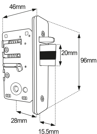
28mm ali latch BL2000 Series
