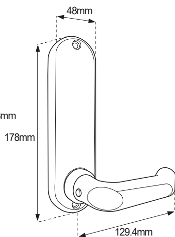
BL5000 ECP Inside handle
