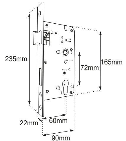
60mm backset euro sash lock
