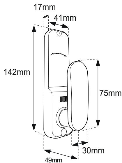
BL2500 ECP - Inside handle
