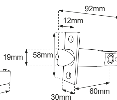
60mm tubular latch
