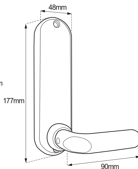
BL5200 ECP - Inside handle
