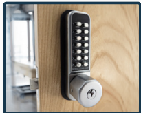
BL2701 ECP FT - Single sided keypad w/ 60mm tubular latch and key override – 60mm tubular latch •Satin Chrome
